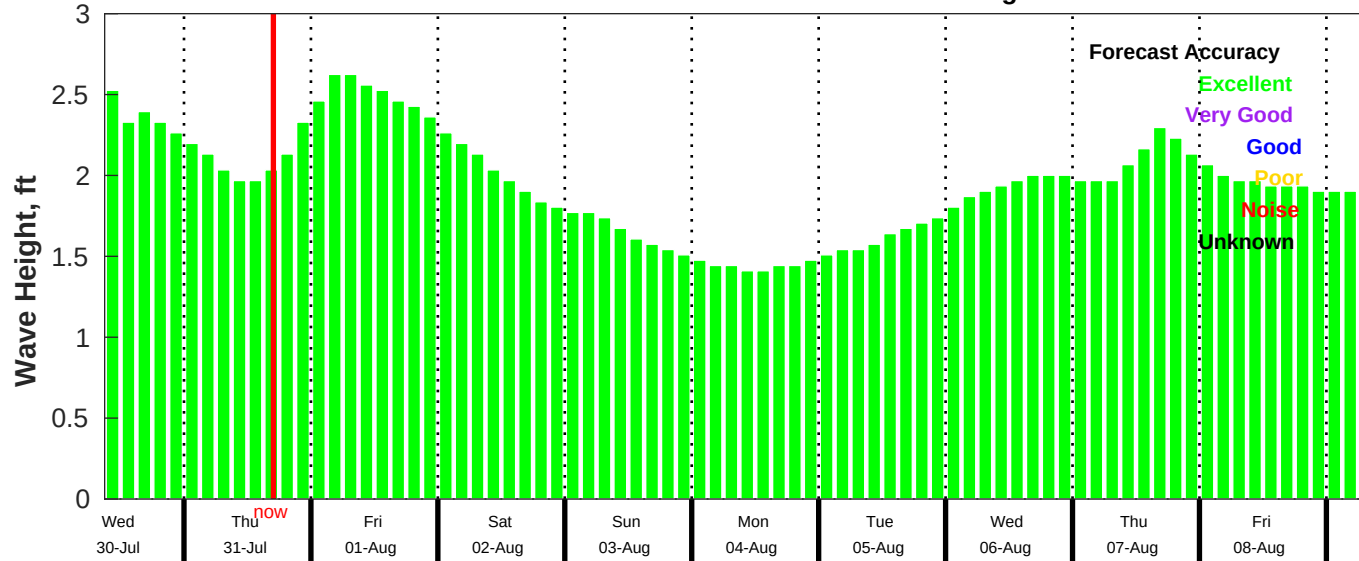
CMEMS Wave Forecast for NDBC 52212 from 29-Jul-2025 09:00:00 to 08-Aug-2025 09:00:00
