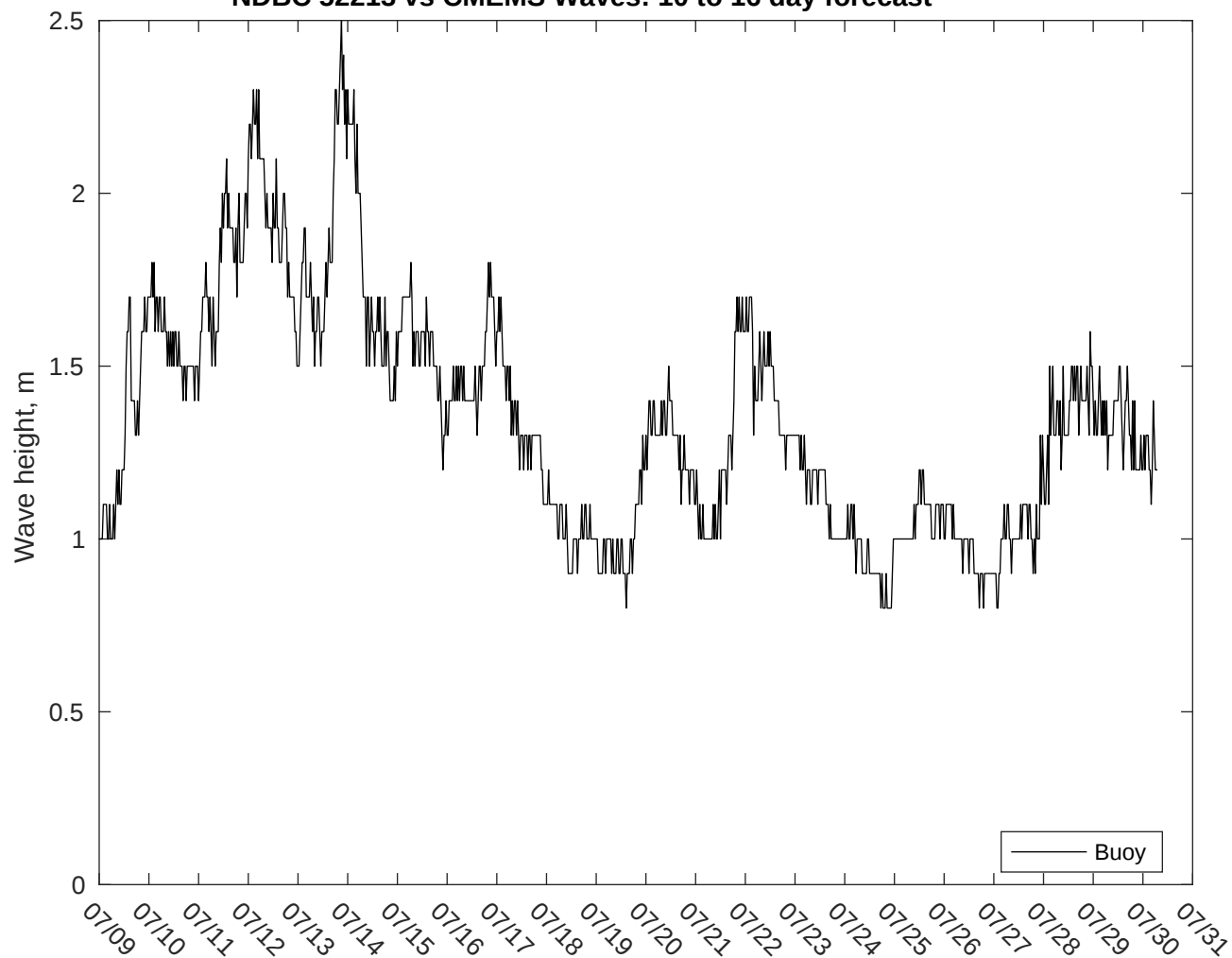
NDBC 52213 vs CMEMS Waves: 10 to 16 day forecast
