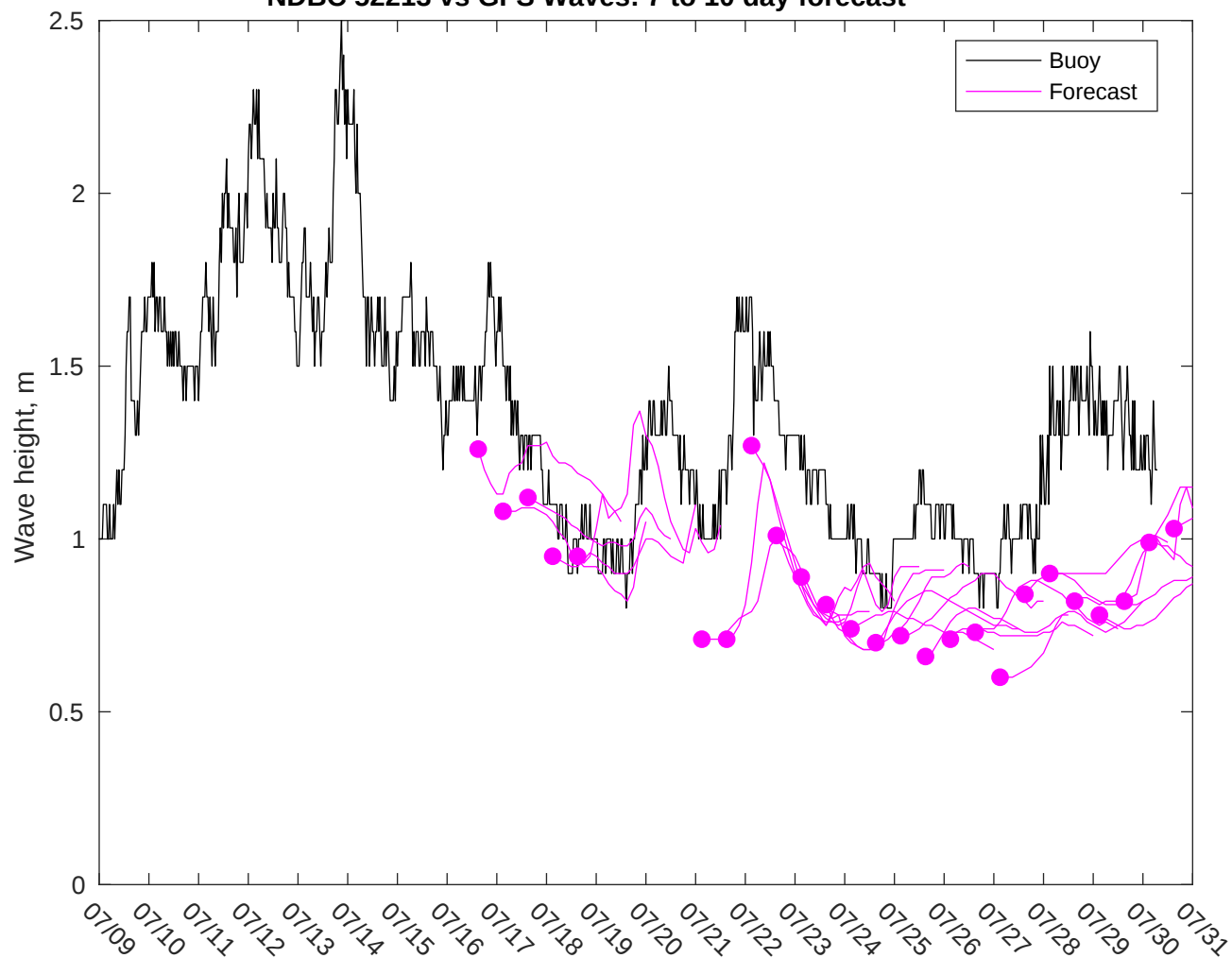
NDBC 52213 vs GFS Waves: 7 to 10 day forecast
