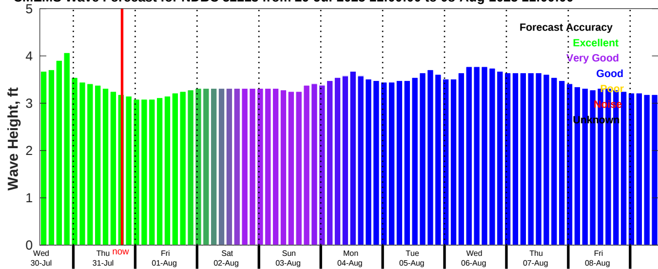
CMEMS Wave Forecast for NDBC 52213 from 29-Jul-2025 11:00:00 to 08-Aug-2025 11:00:00
