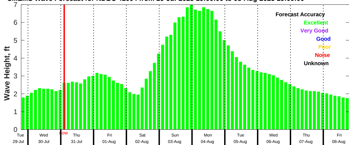
CMEMS Wave Forecast for NDBC 41004 from 29-Jul-2025 19:00:00 to 08-Aug-2025 19:00:00
