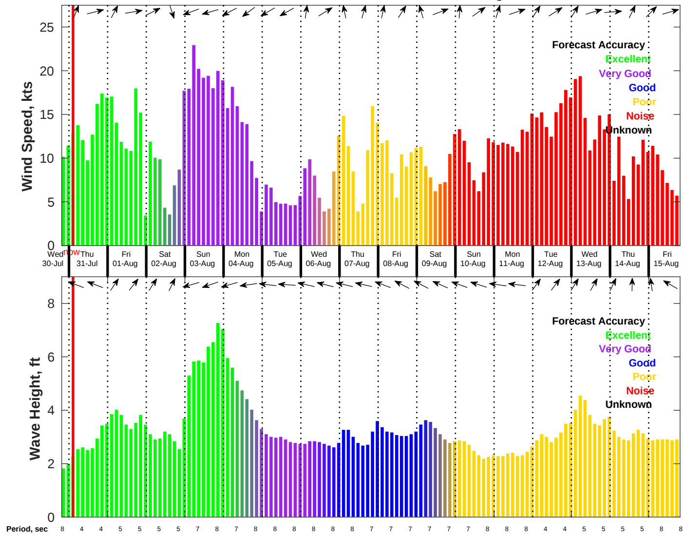
Wind & Wave Forecast for NDBC 41004 from 30-Jul-2025 19:00:00 to 15-Aug-2025 19:00:00
