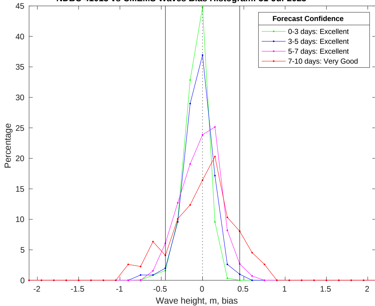
NDBC 41013 vs CMEMS Waves Bias Histogram: 31-Jul-2025
