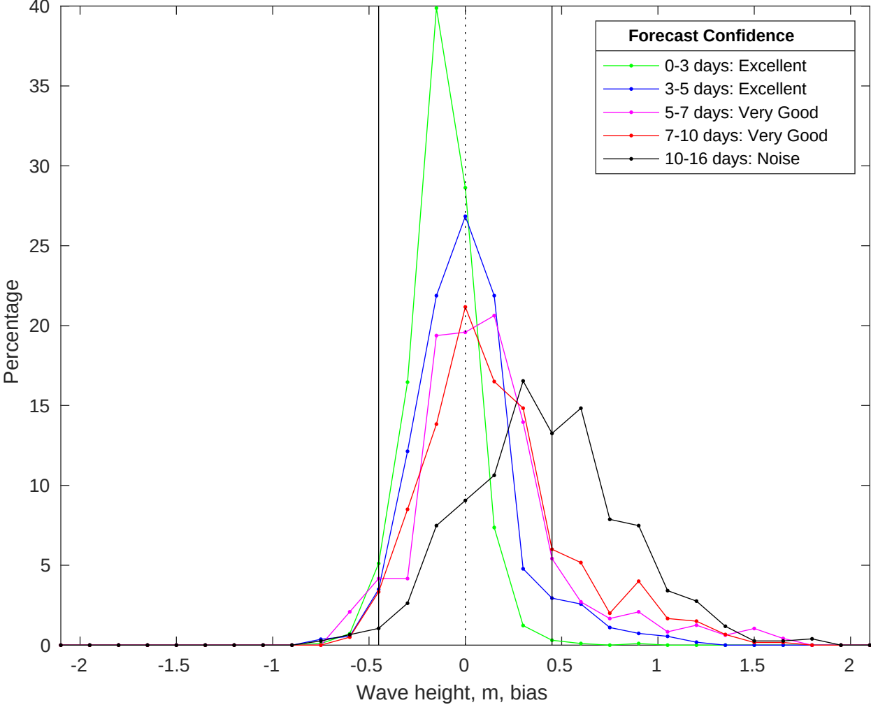
NDBC 41013 vs GFS Waves Bias Histogram: 31-Jul-2025
