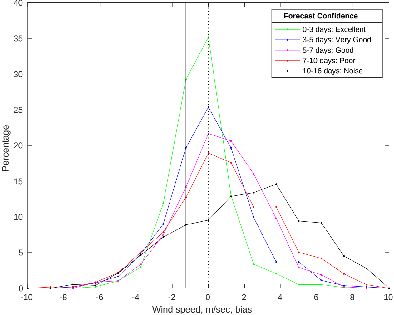
NDBC 41013 vs GFS Winds Bias Histogram: 31-Jul-2025
