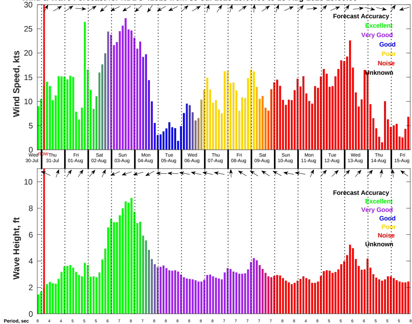
Wind & Wave Forecast for NDBC 41013 from 30-Jul-2025 19:00:00 to 15-Aug-2025 19:00:00
