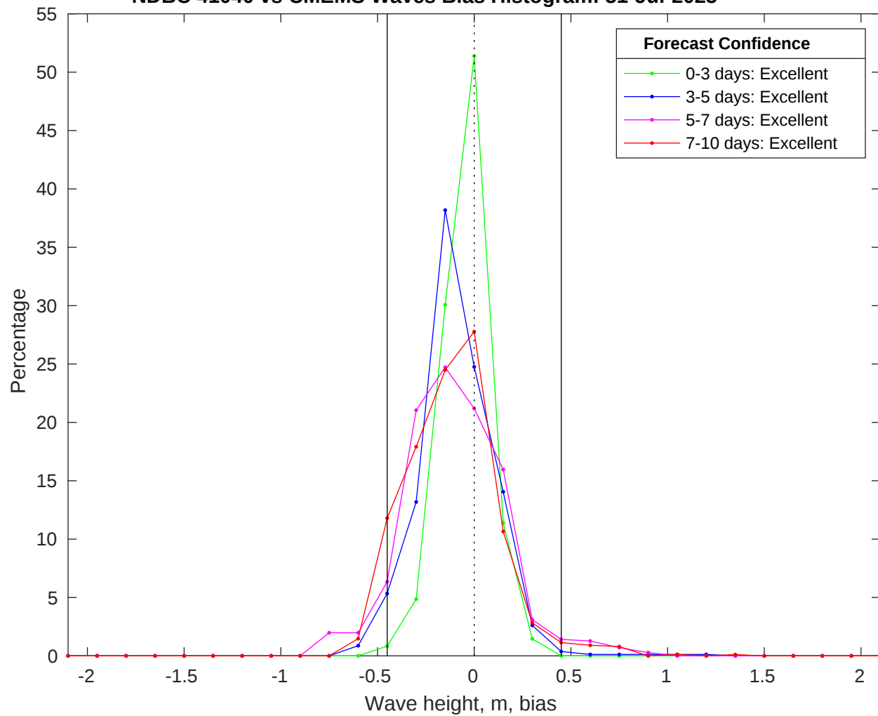
NDBC 41040 vs CMEMS Waves Bias Histogram: 31-Jul-2025
