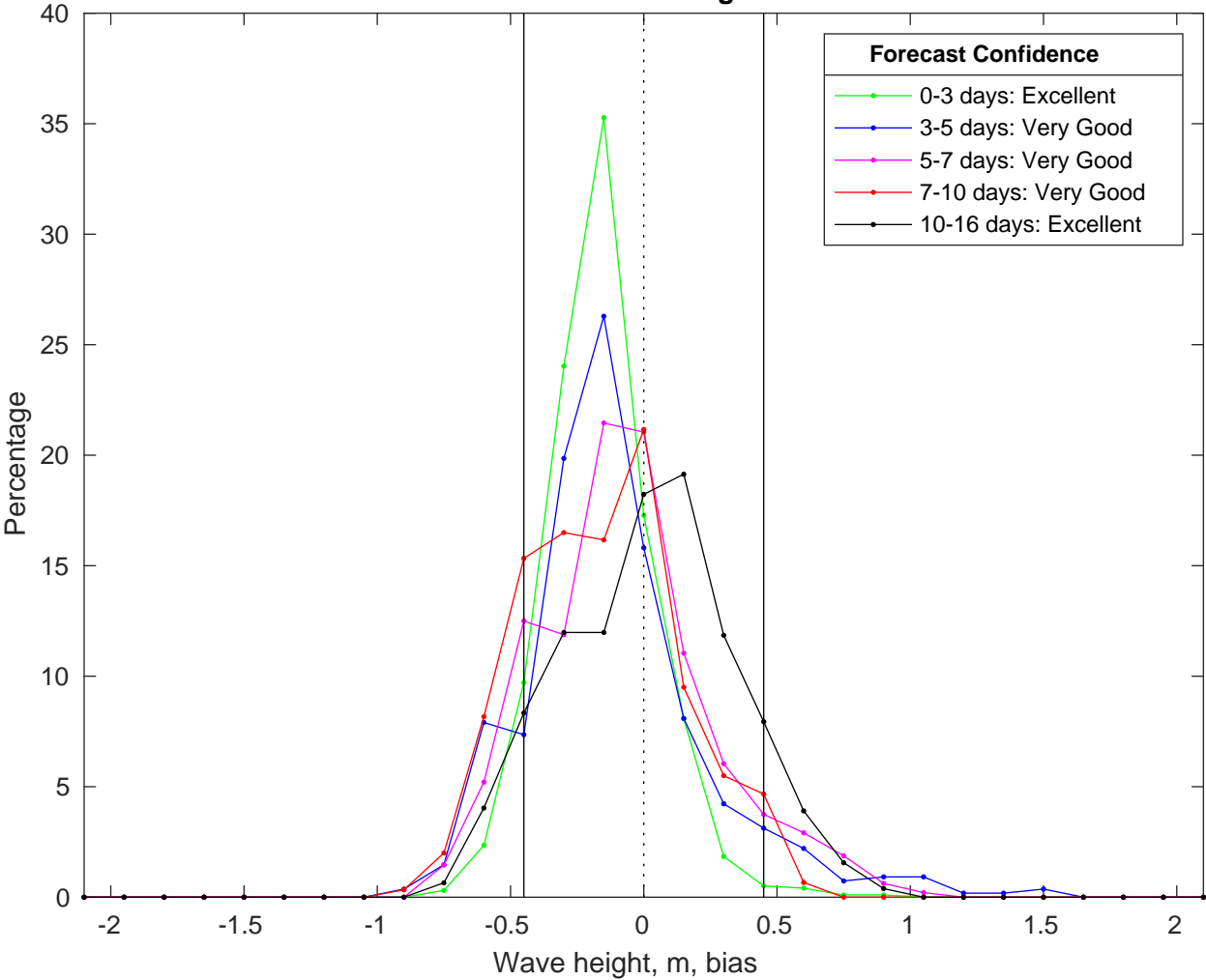
NDBC 41040 vs GFS Waves Bias Histogram: 31-Jul-2025
