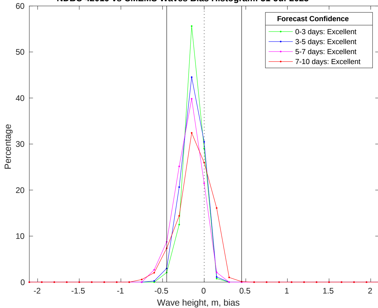
NDBC 42019 vs CMEMS Waves Bias Histogram: 31-Jul-2025
