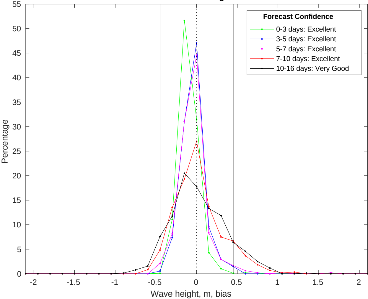
NDBC 42019 vs GFS Waves Bias Histogram: 31-Jul-2025
