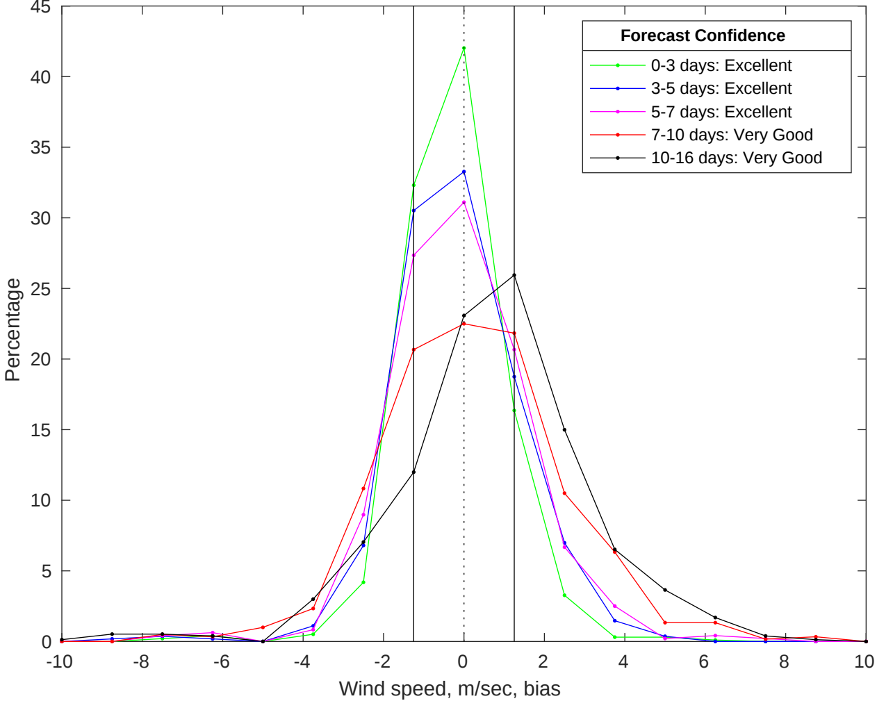
NDBC 42019 vs GFS Winds Bias Histogram: 31-Jul-2025
