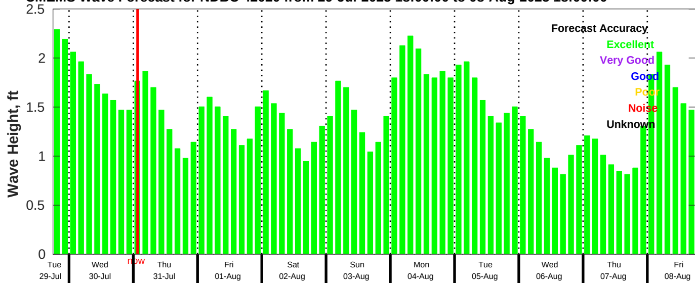
CMEMS Wave Forecast for NDBC 42020 from 29-Jul-2025 18:00:00 to 08-Aug-2025 18:00:00
