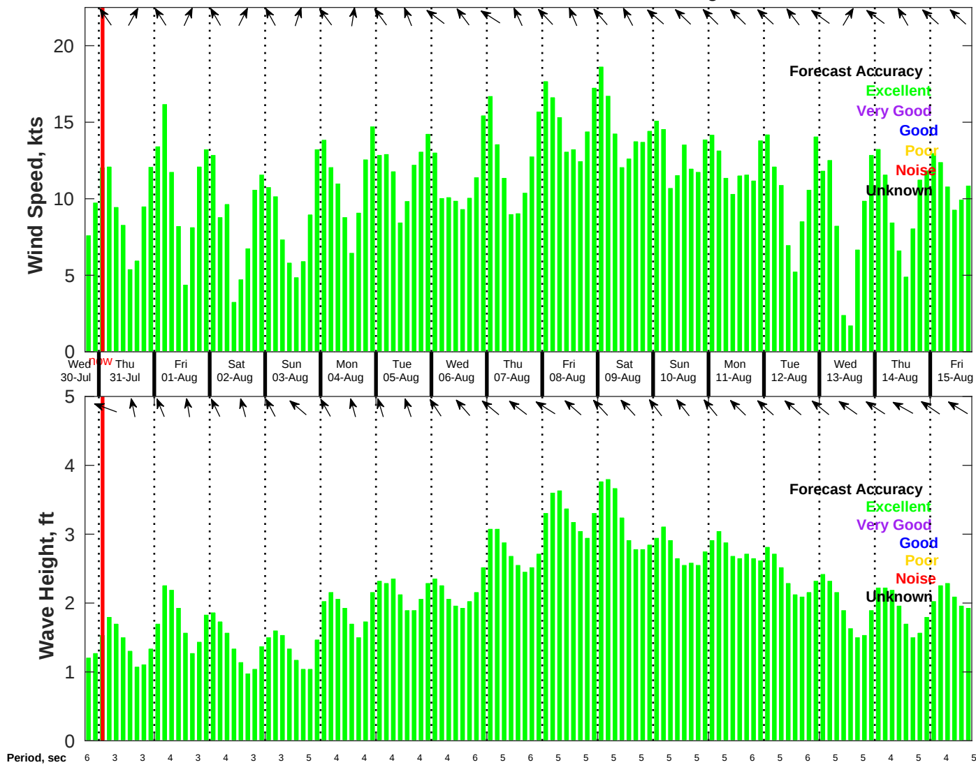
Wind & Wave Forecast for NDBC 42020 from 30-Jul-2025 18:00:00 to 15-Aug-2025 18:00:00
