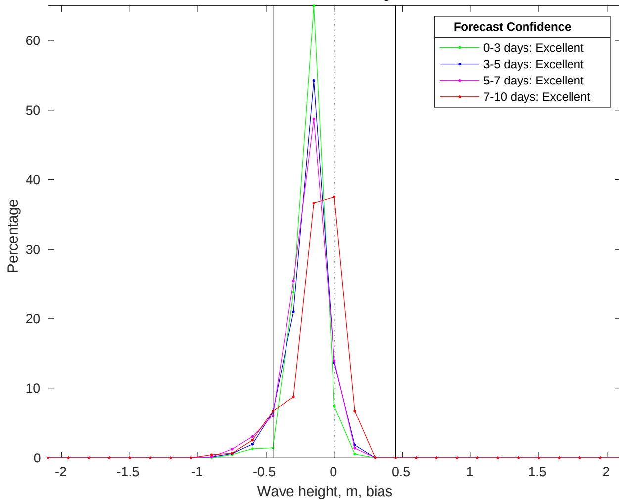
NDBC 42035 vs CMEMS Waves Bias Histogram: 31-Jul-2025
