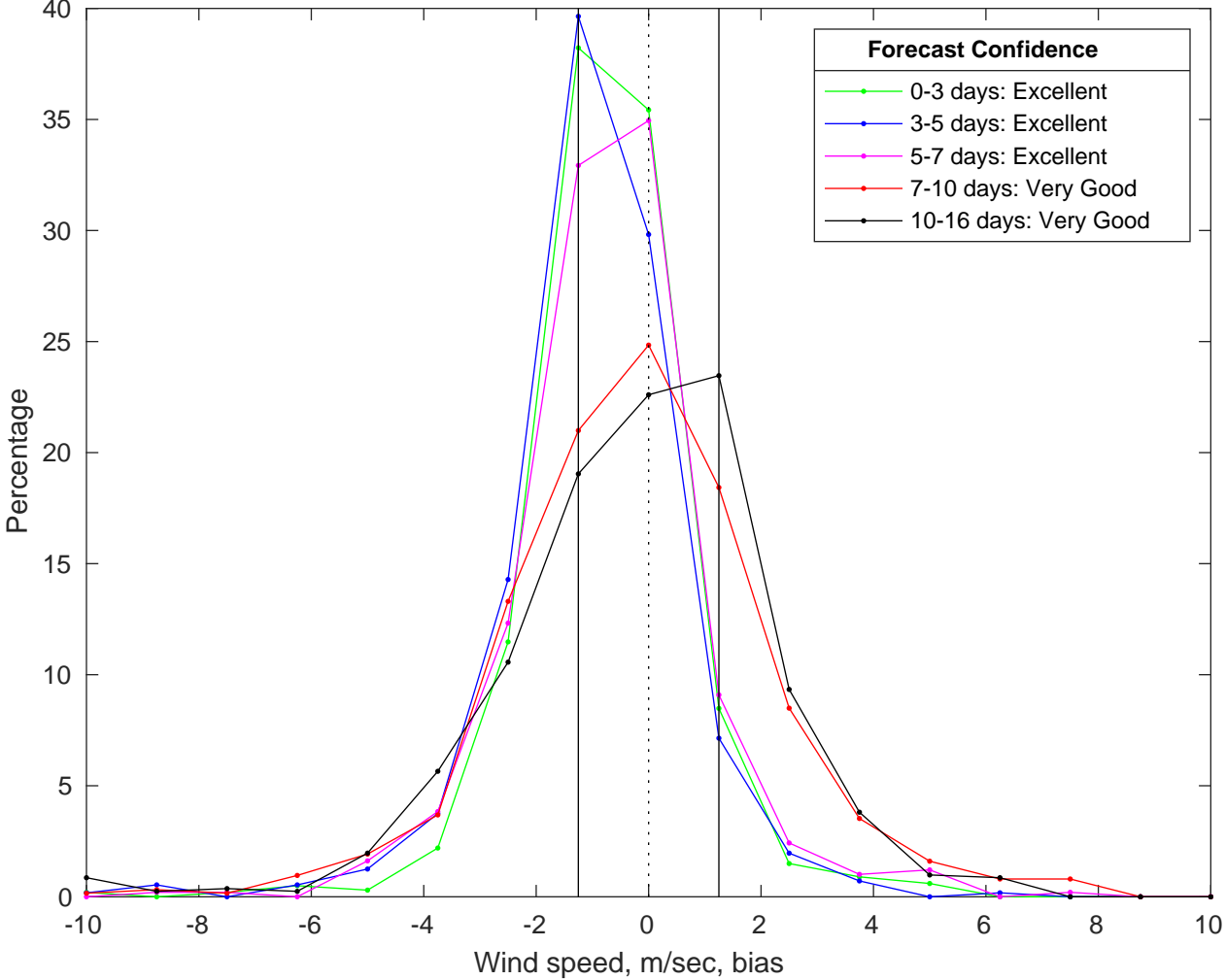
NDBC 42035 vs GFS Winds Bias Histogram: 31-Jul-2025
