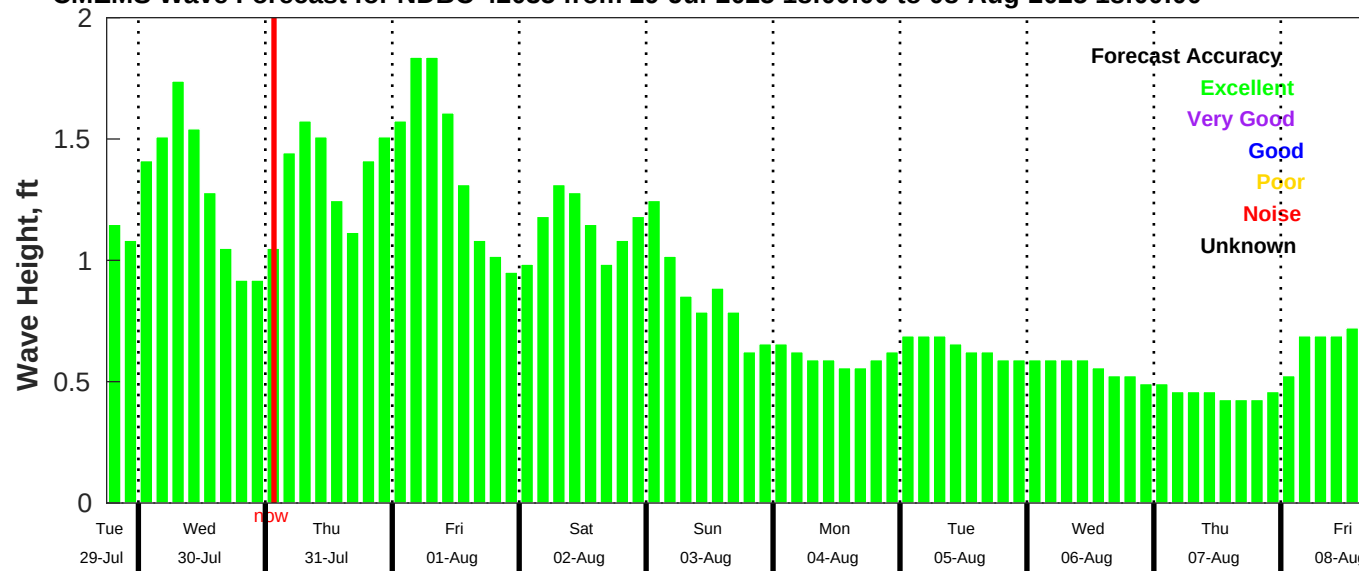
CMEMS Wave Forecast for NDBC 42035 from 29-Jul-2025 18:00:00 to 08-Aug-2025 18:00:00
