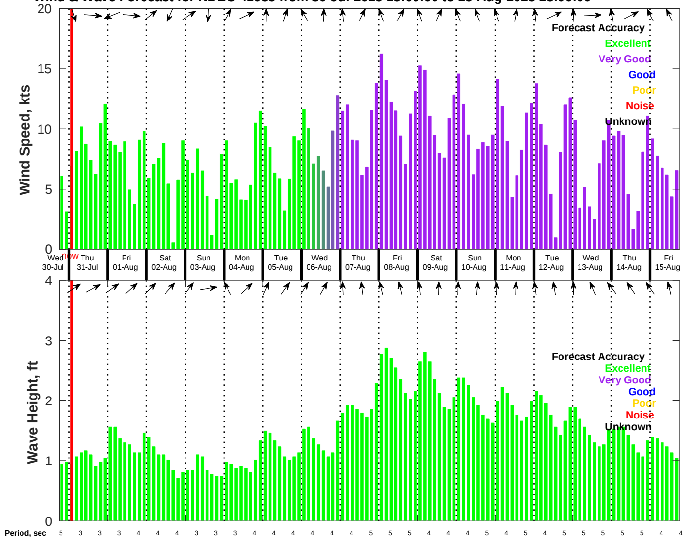
Wind & Wave Forecast for NDBC 42035 from 30-Jul-2025 18:00:00 to 15-Aug-2025 18:00:00
