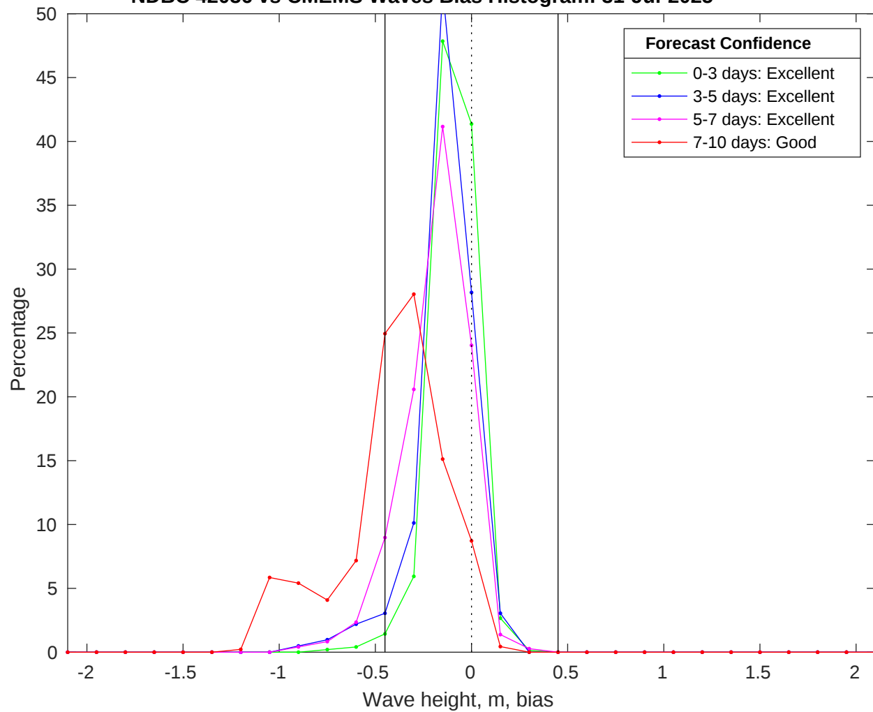
NDBC 42036 vs CMEMS Waves Bias Histogram: 31-Jul-2025
