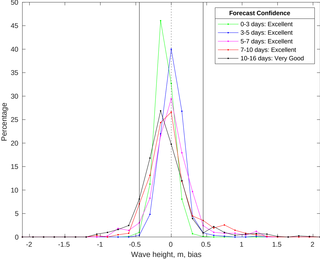
NDBC 42036 vs GFS Waves Bias Histogram: 31-Jul-2025
