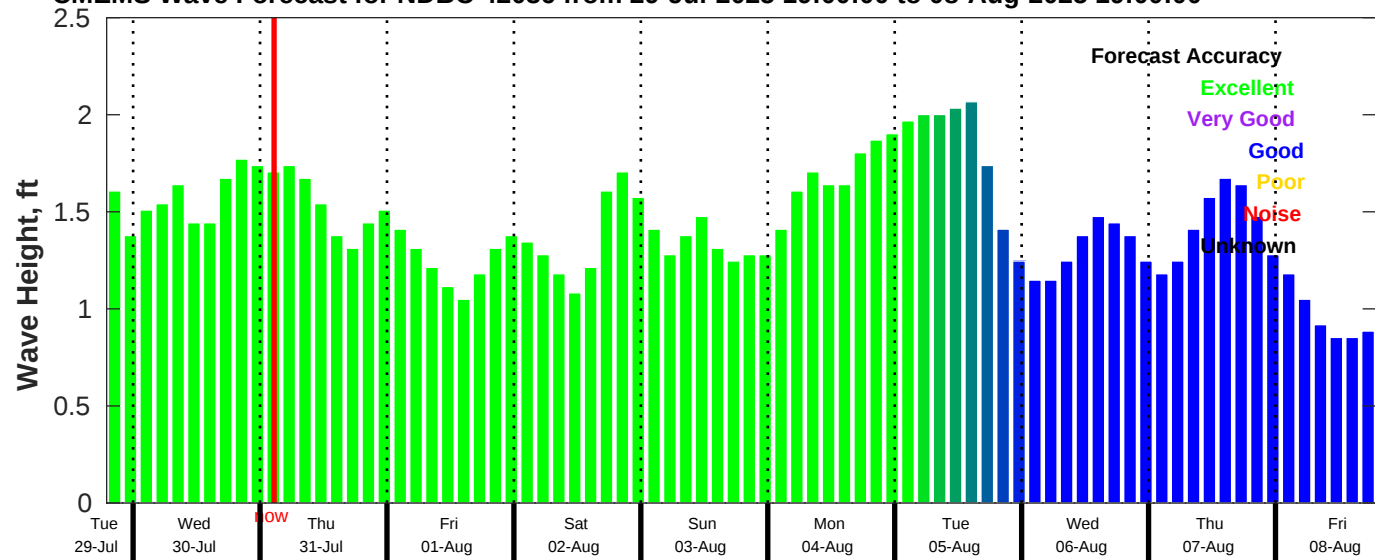
CMEMS Wave Forecast for NDBC 42036 from 29-Jul-2025 19:00:00 to 08-Aug-2025 19:00:00
