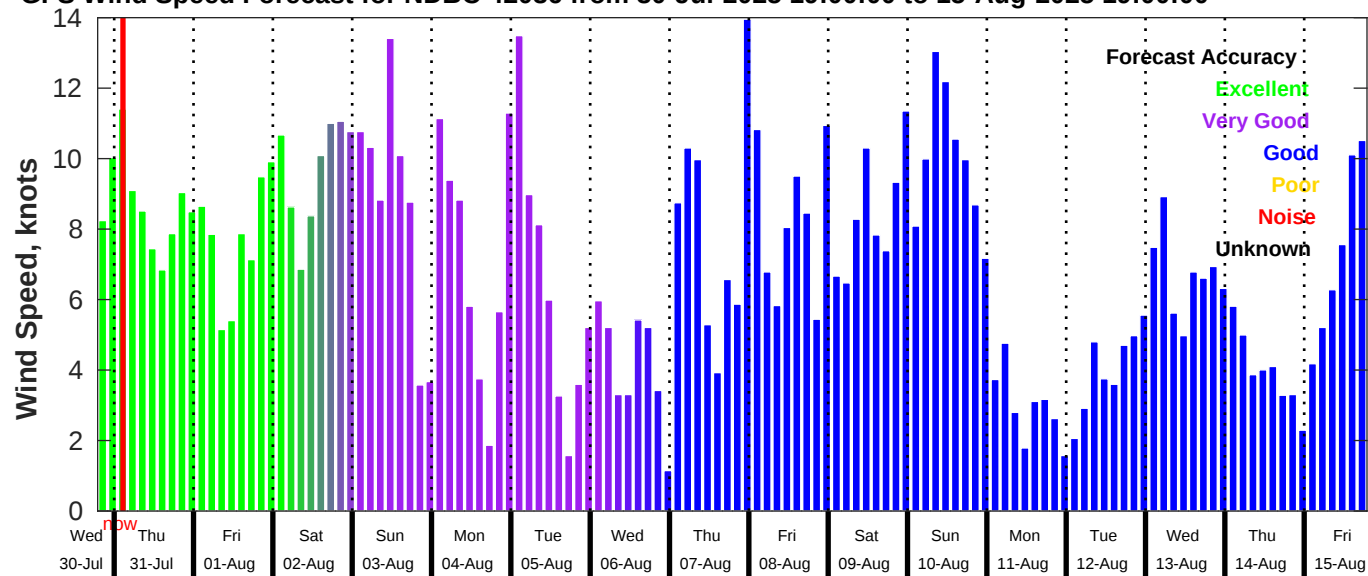
GFS Wind Speed Forecast for NDBC 42036 from 30-Jul-2025 19:00:00 to 15-Aug-2025 19:00:00
