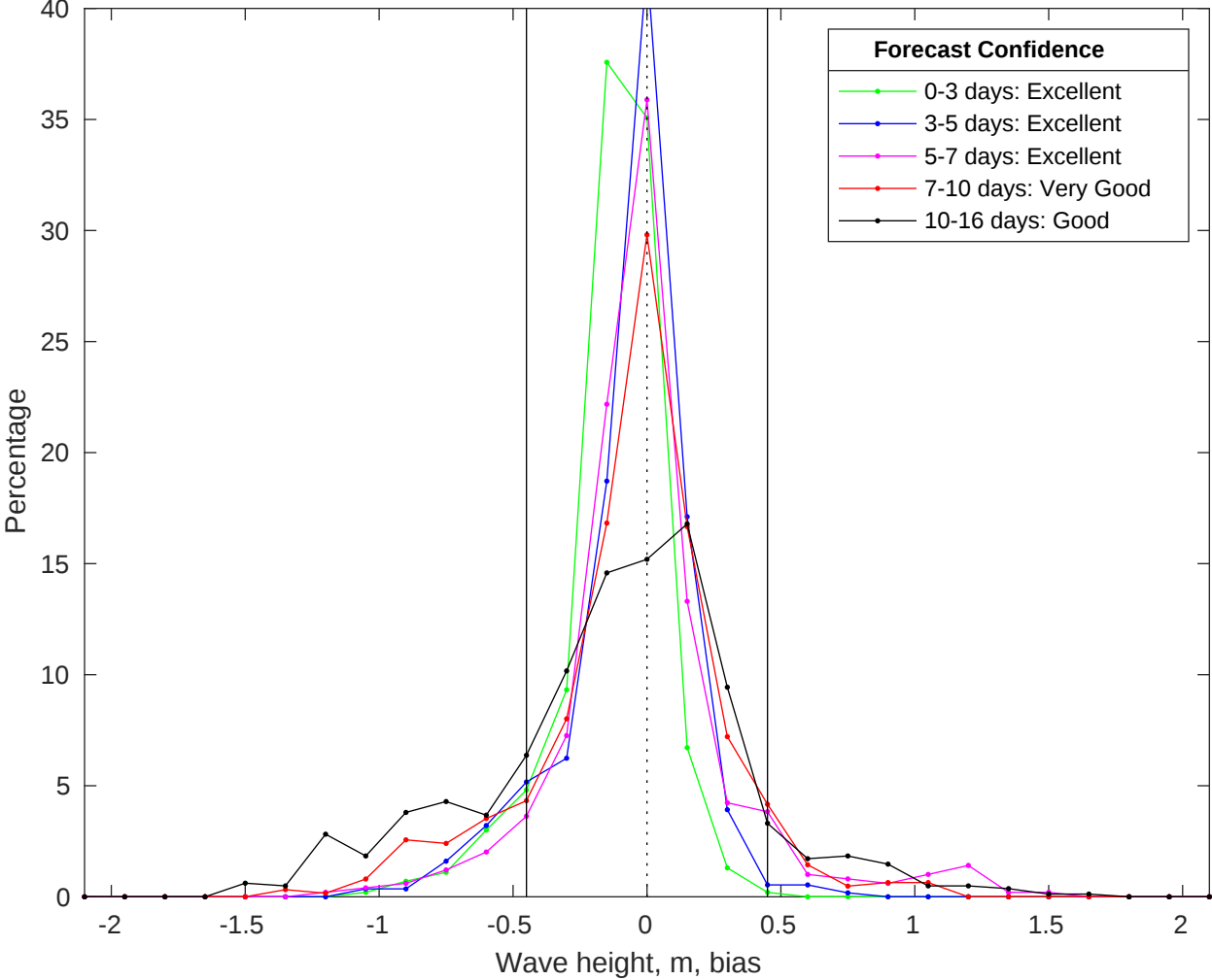
NDBC 42040 vs GFS Waves Bias Histogram: 31-Jul-2025
