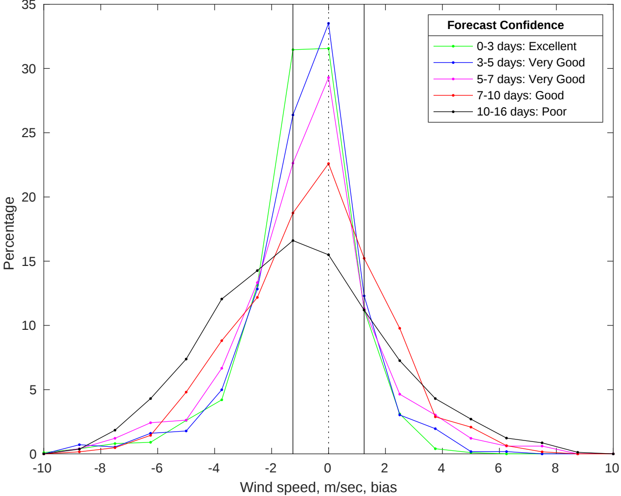
NDBC 42040 vs GFS Winds Bias Histogram: 31-Jul-2025
