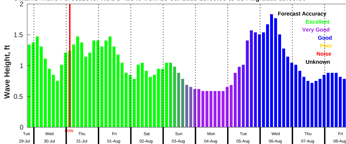
CMEMS Wave Forecast for NDBC 42040 from 29-Jul-2025 19:00:00 to 08-Aug-2025 19:00:00
