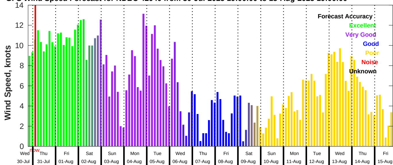
GFS Wind Speed Forecast for NDBC 42040 from 30-Jul-2025 19:00:00 to 15-Aug-2025 19:00:00
