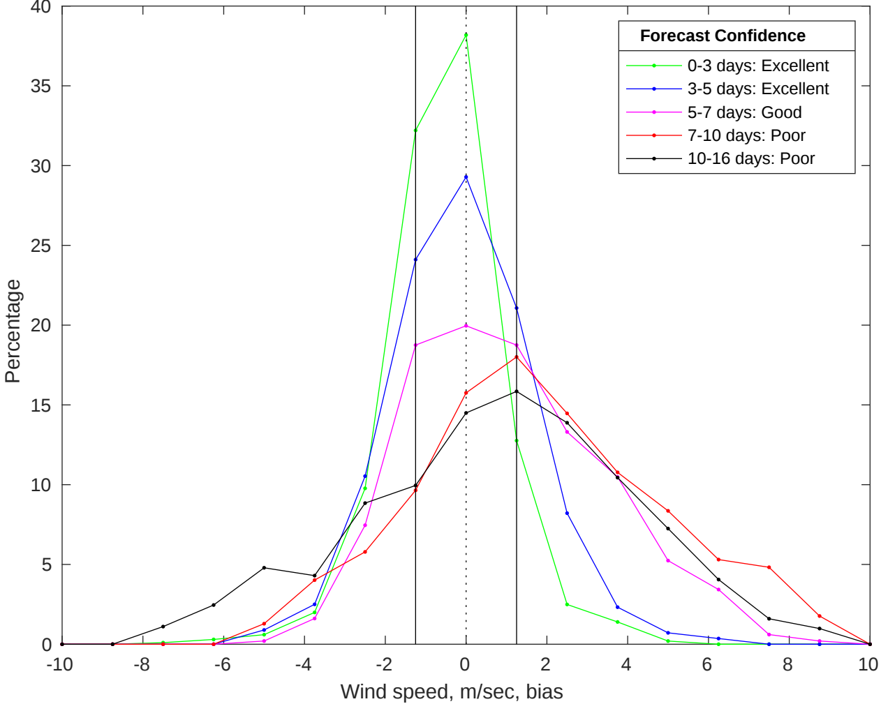
NDBC 46011 vs GFS Winds Bias Histogram: 31-Jul-2025
