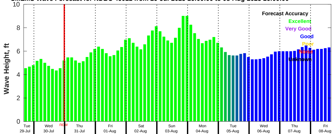
CMEMS Wave Forecast for NDBC 46011 from 29-Jul-2025 16:00:00 to 08-Aug-2025 16:00:00
