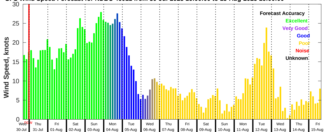
GFS Wind Speed Forecast for NDBC 46011 from 30-Jul-2025 16:00:00 to 15-Aug-2025 16:00:00
