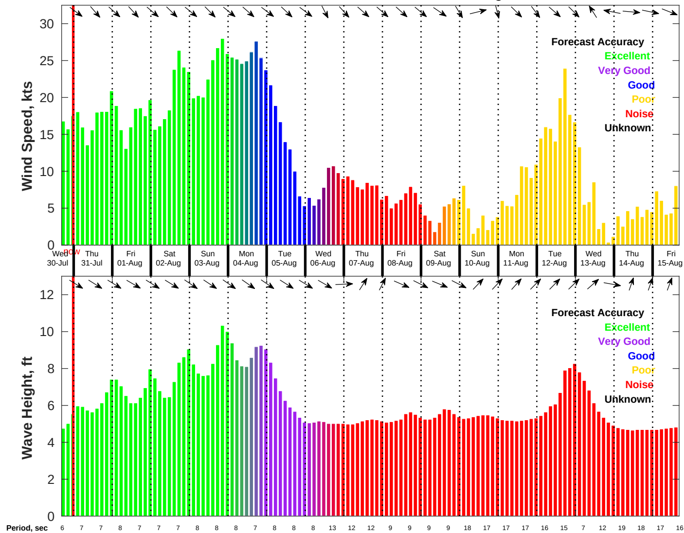
Wind & Wave Forecast for NDBC 46011 from 30-Jul-2025 16:00:00 to 15-Aug-2025 16:00:00
