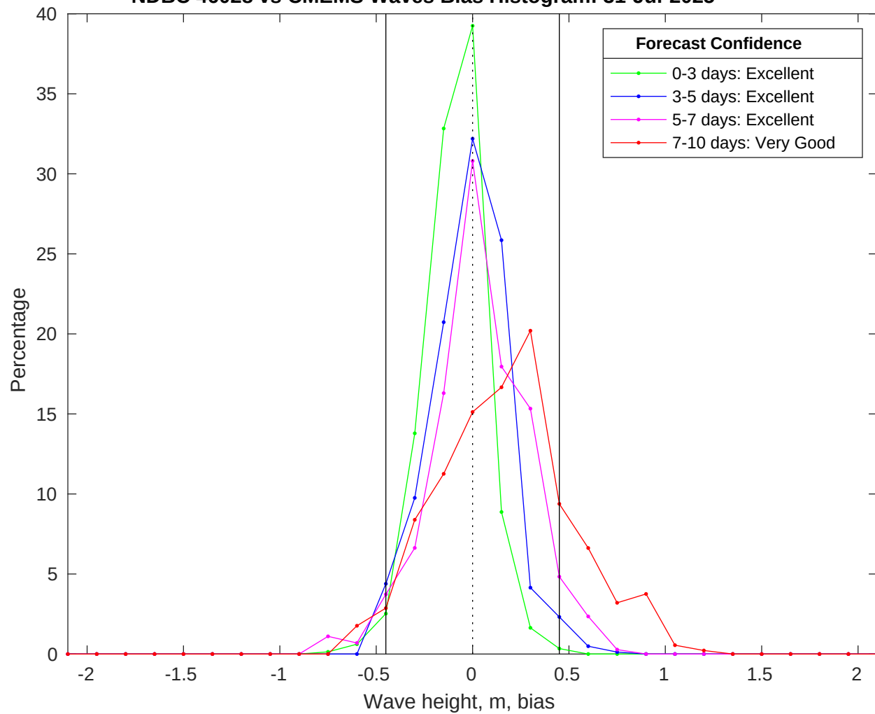
NDBC 46028 vs CMEMS Waves Bias Histogram: 31-Jul-2025
