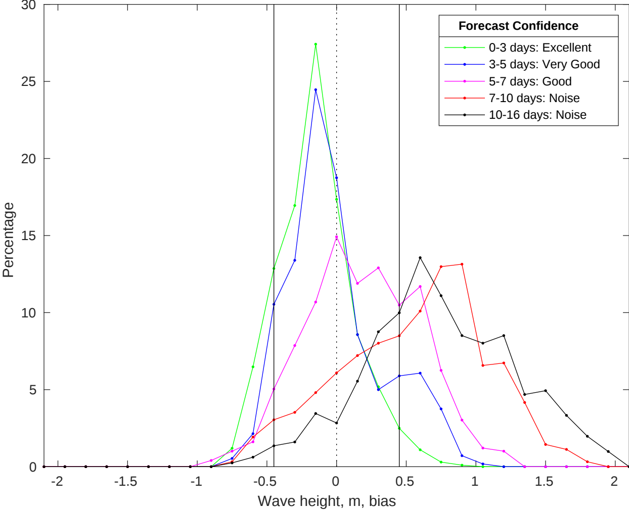
NDBC 46028 vs GFS Waves Bias Histogram: 31-Jul-2025
