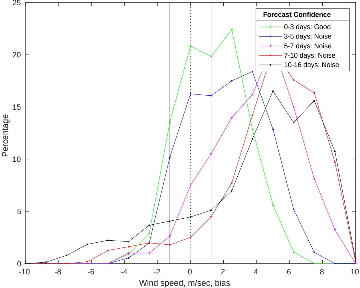
NDBC 46028 vs GFS Winds Bias Histogram: 31-Jul-2025
