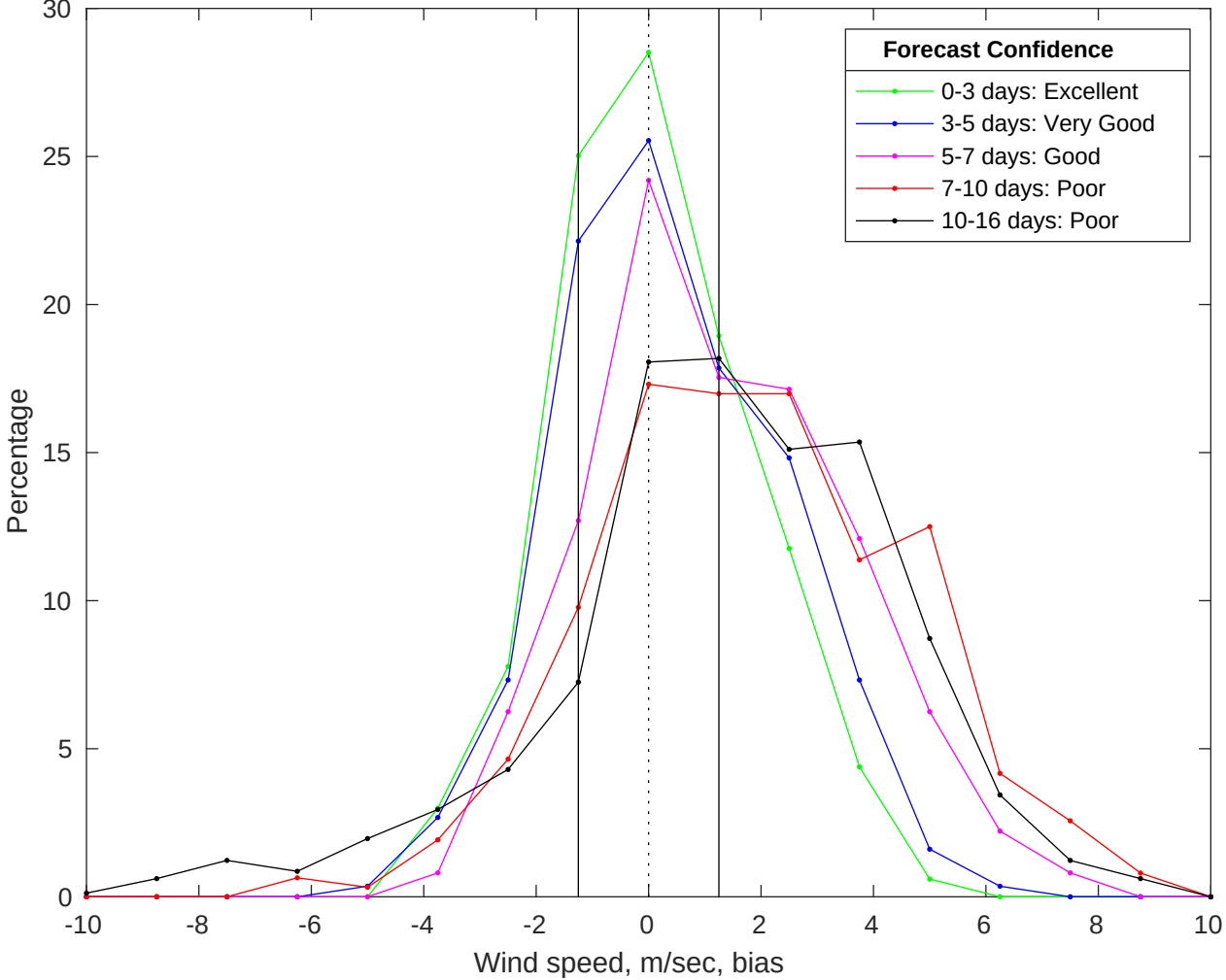
NDBC 46054 vs GFS Winds Bias Histogram: 31-Jul-2025
