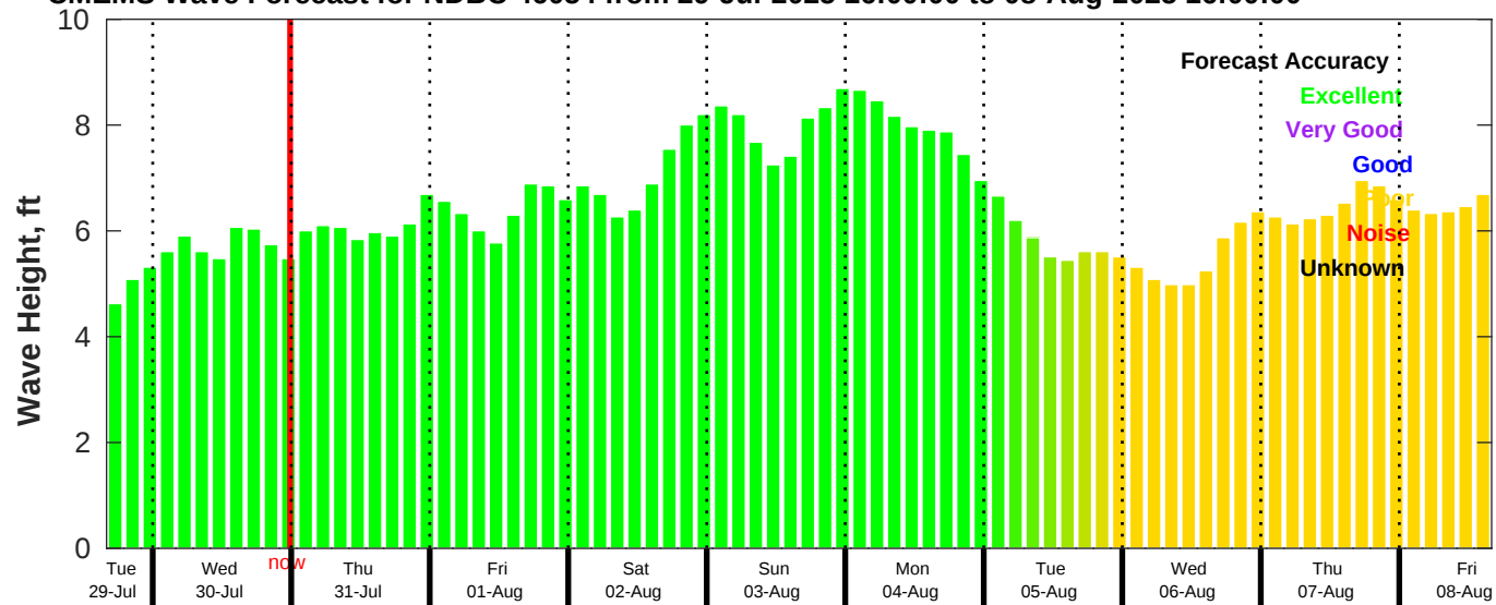
CMEMS Wave Forecast for NDBC 46054 from 29-Jul-2025 16:00:00 to 08-Aug-2025 16:00:00
