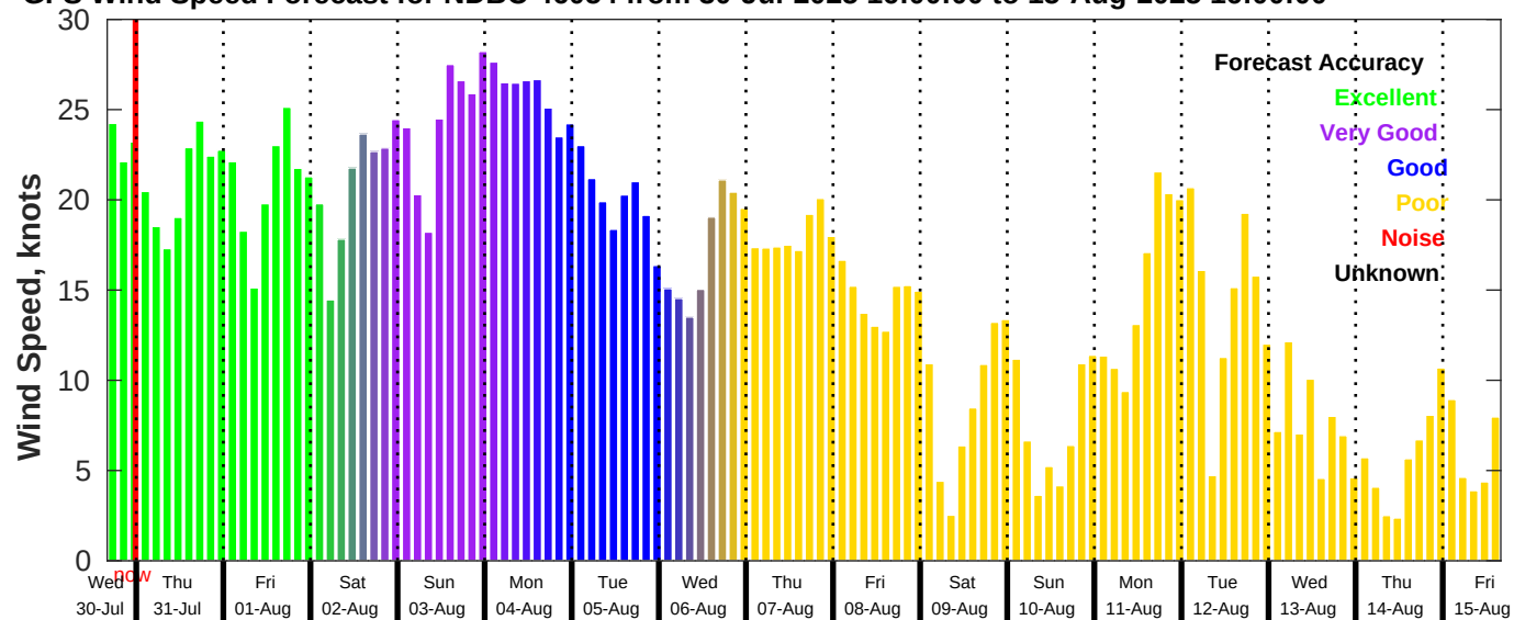
GFS Wind Speed Forecast for NDBC 46054 from 30-Jul-2025 16:00:00 to 15-Aug-2025 16:00:00
