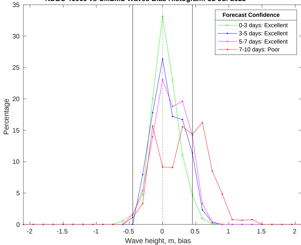
NDBC 46069 vs CMEMS Waves Bias Histogram: 31-Jul-2025
