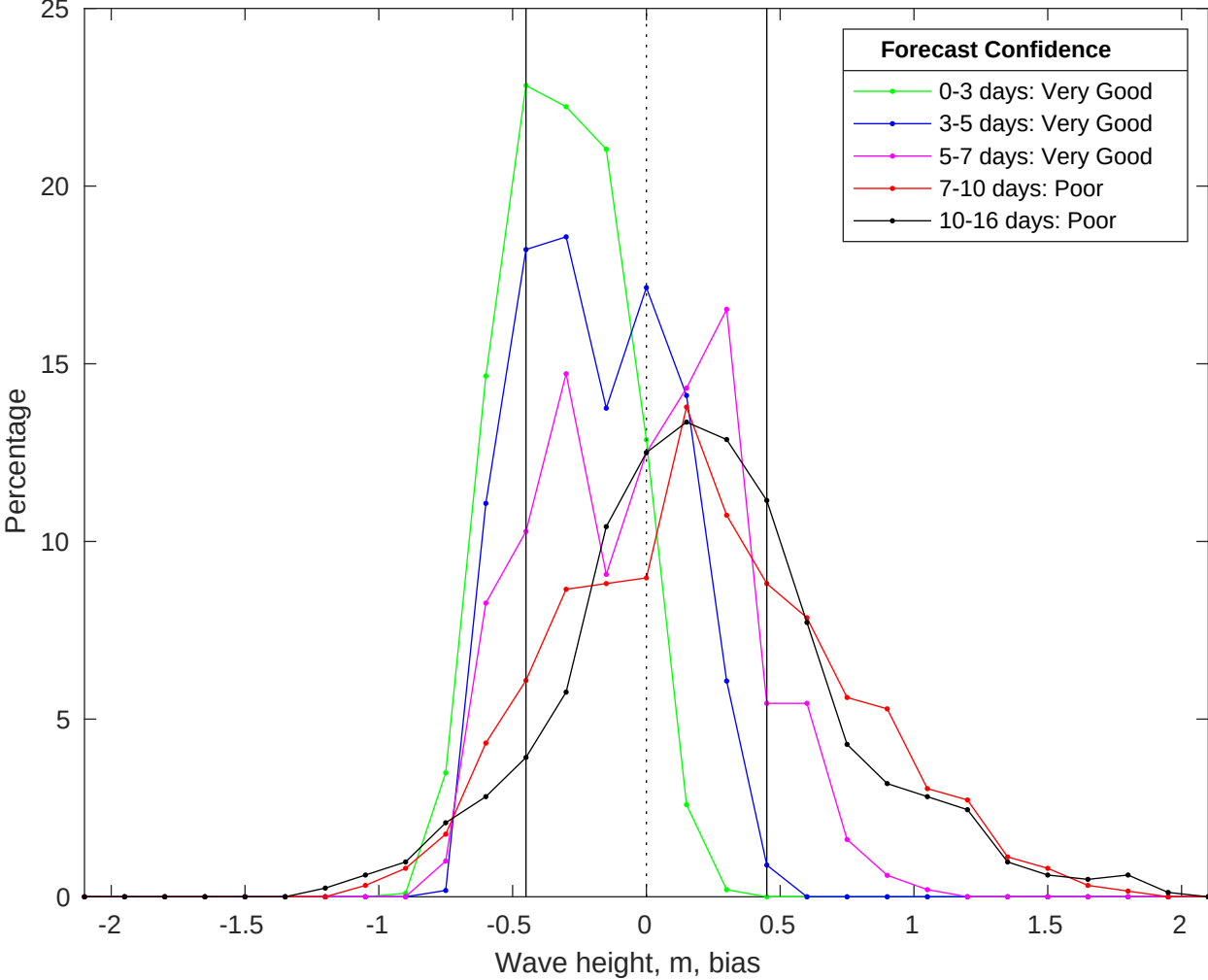
NDBC 46069 vs GFS Waves Bias Histogram: 31-Jul-2025
