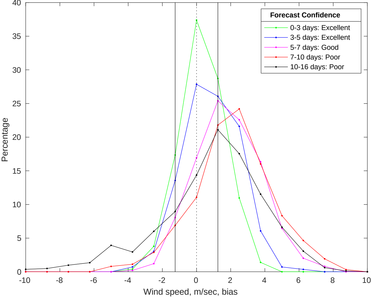
NDBC 46069 vs GFS Winds Bias Histogram: 31-Jul-2025
