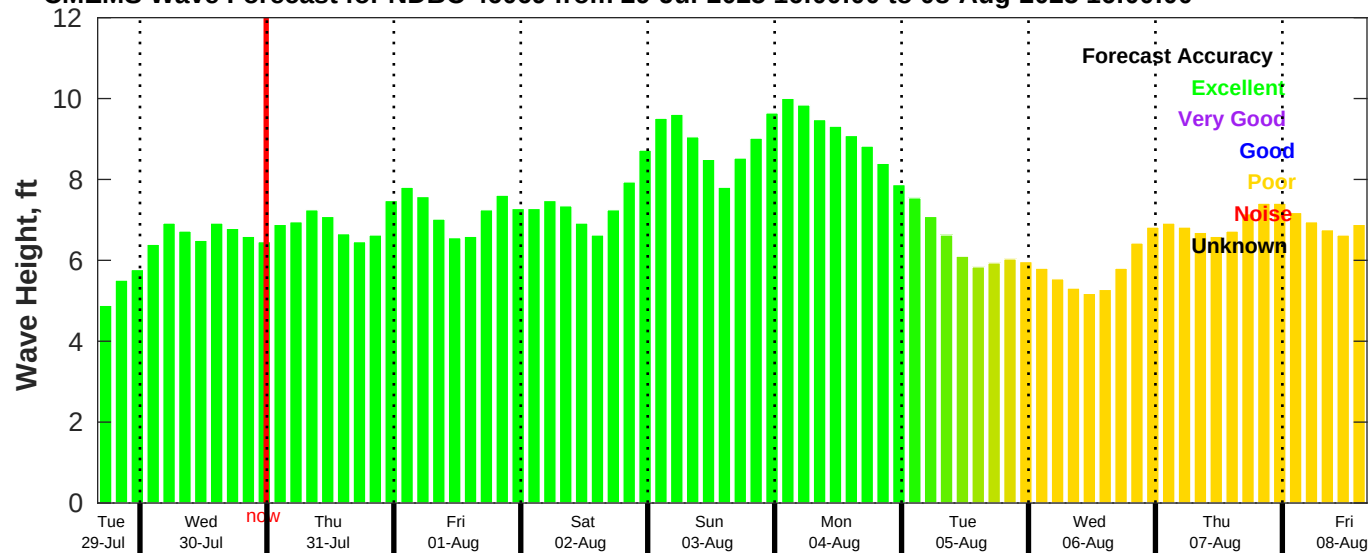
CMEMS Wave Forecast for NDBC 46069 from 29-Jul-2025 16:00:00 to 08-Aug-2025 16:00:00
