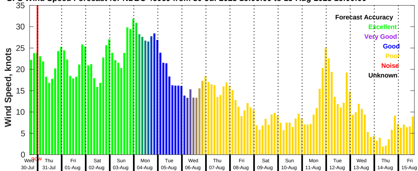
GFS Wind Speed Forecast for NDBC 46069 from 30-Jul-2025 16:00:00 to 15-Aug-2025 16:00:00
