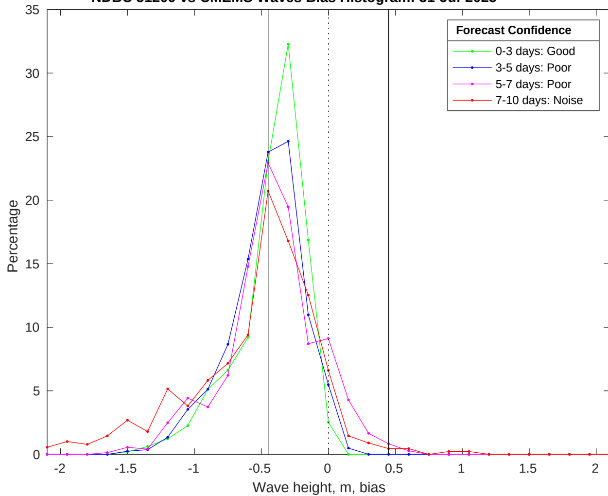
NDBC 51209 vs CMEMS Waves Bias Histogram: 31-Jul-2025
