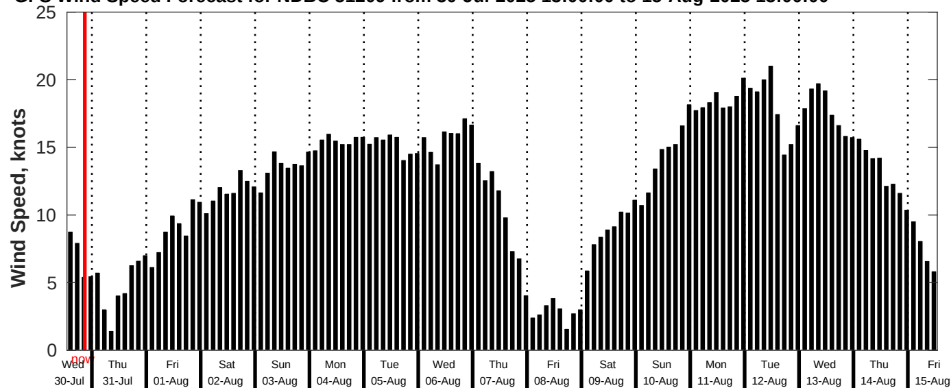
GFS Wind Speed Forecast for NDBC 51209 from 30-Jul-2025 13:00:00 to 15-Aug-2025 13:00:00
