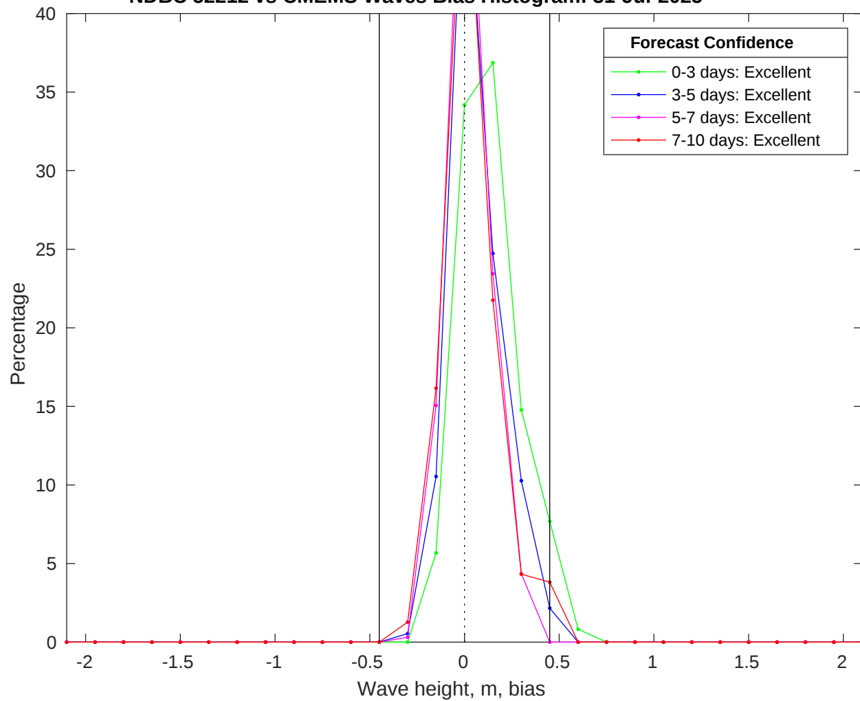
NDBC 52212 vs CMEMS Waves Bias Histogram: 31-Jul-2025
