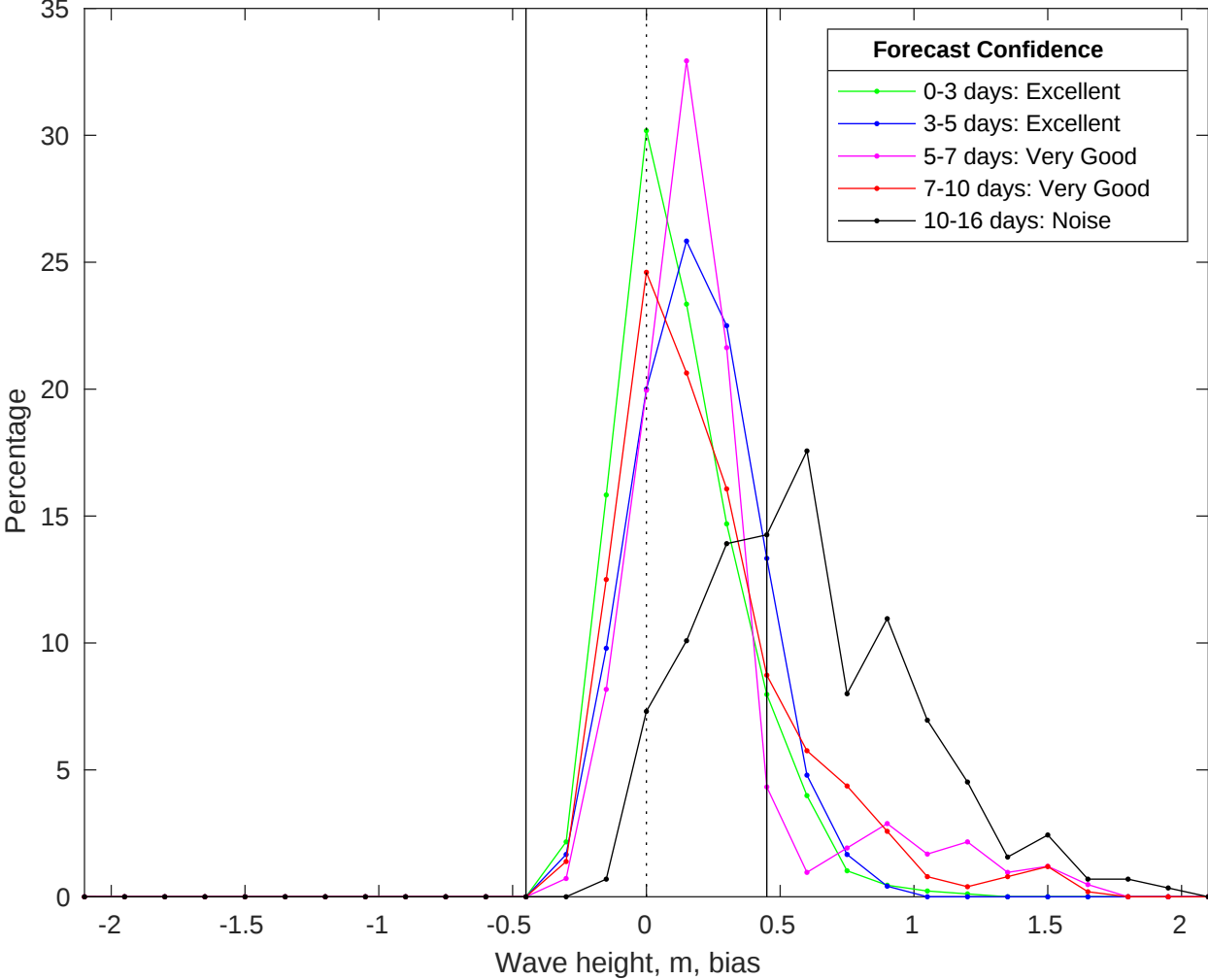
NDBC 52212 vs GFS Waves Bias Histogram: 31-Jul-2025
