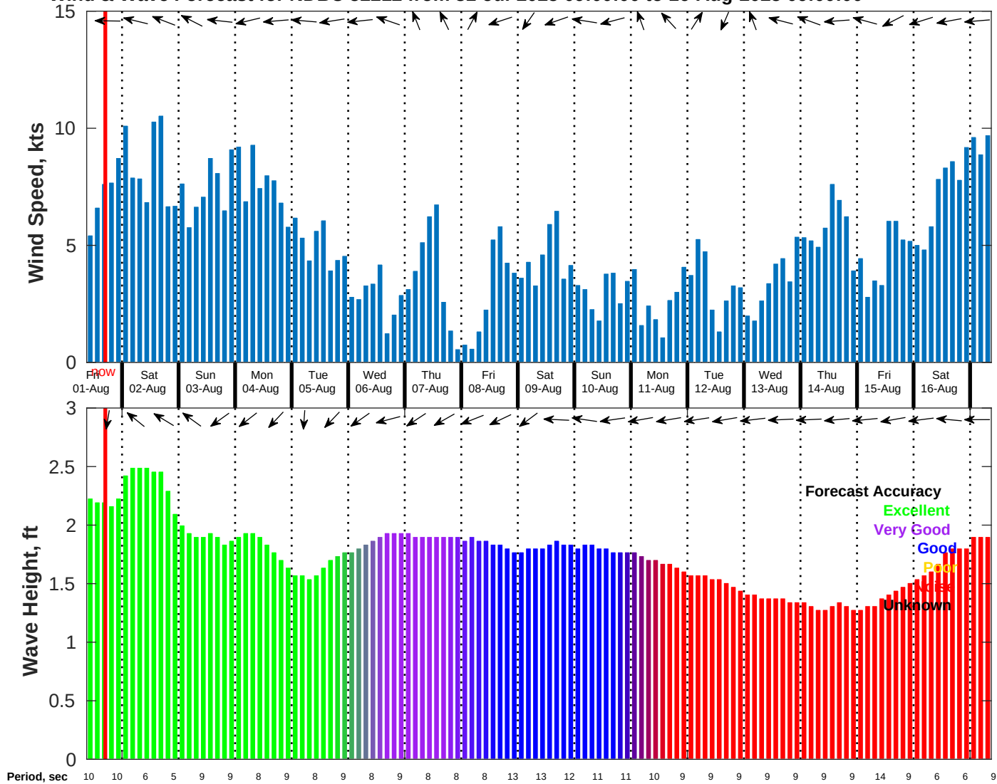
Wind & Wave Forecast for NDBC 52212 from 31-Jul-2025 09:00:00 to 16-Aug-2025 09:00:00
