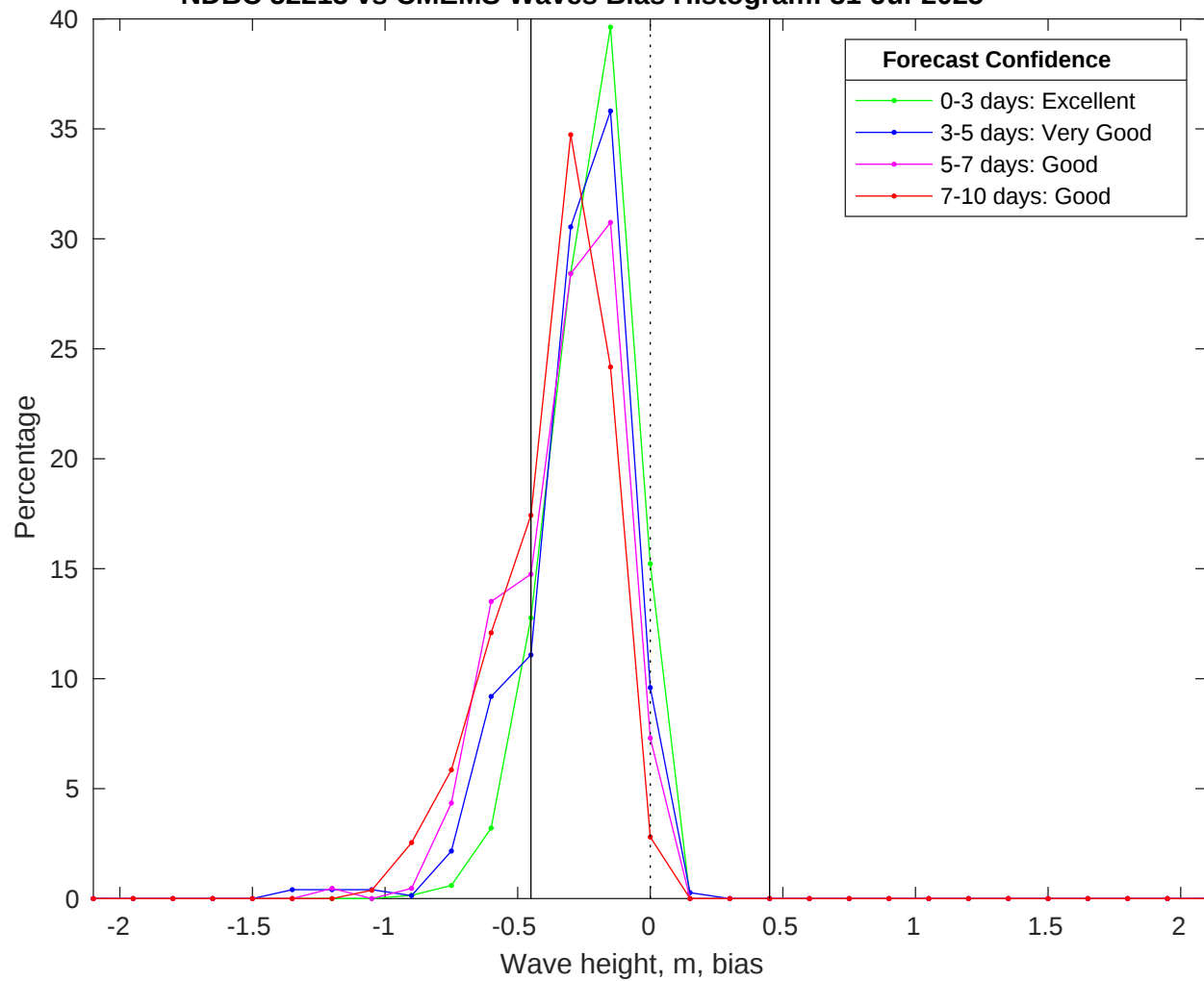
NDBC 52213 vs CMEMS Waves Bias Histogram: 31-Jul-2025
